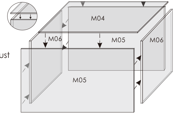
scale 1:4 M06 Transparent cover 21*18.5*0.15cm 2 pieces
